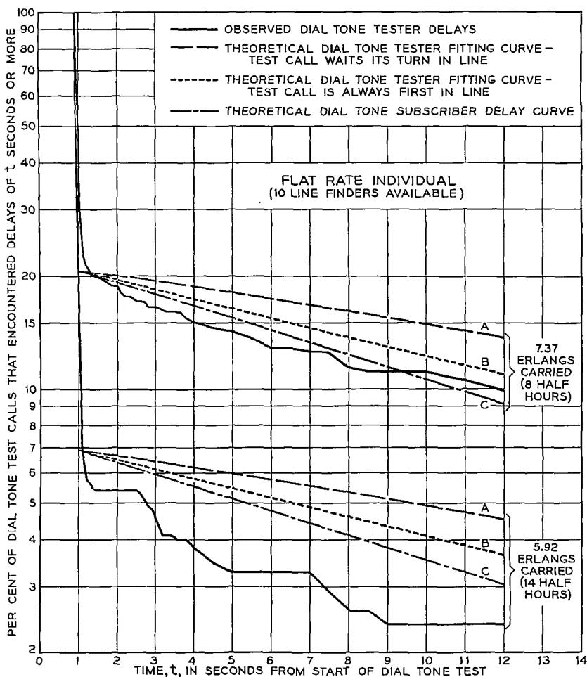
Fig. 5—Results of dial tone tests.
