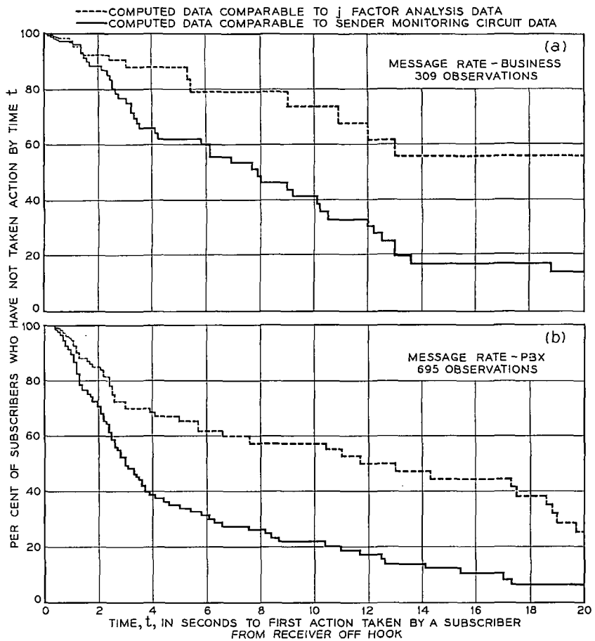
Fig. 18—Subscriber dialing habits based on individual line records when dial tone is delayed indefinitely.
